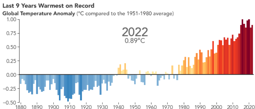
Figure 55: Global Temperature 1880-2022 172
