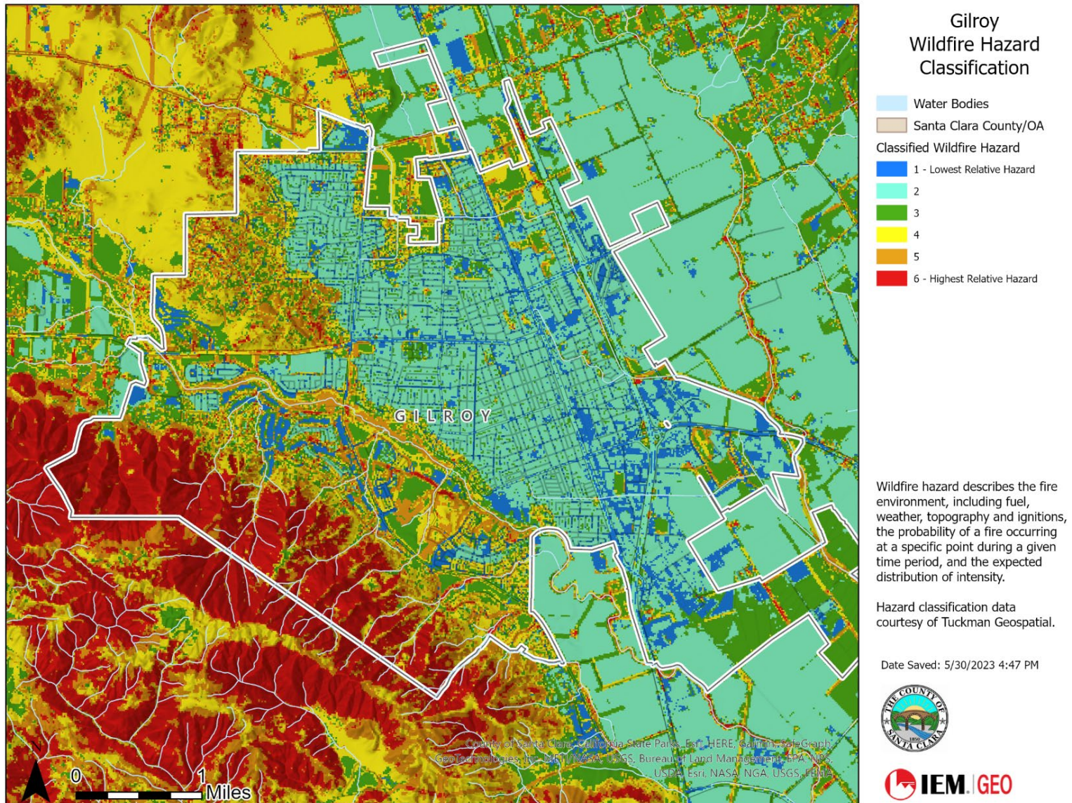
Figure 36: City of Gilroy Wildfire Hazard Classification
