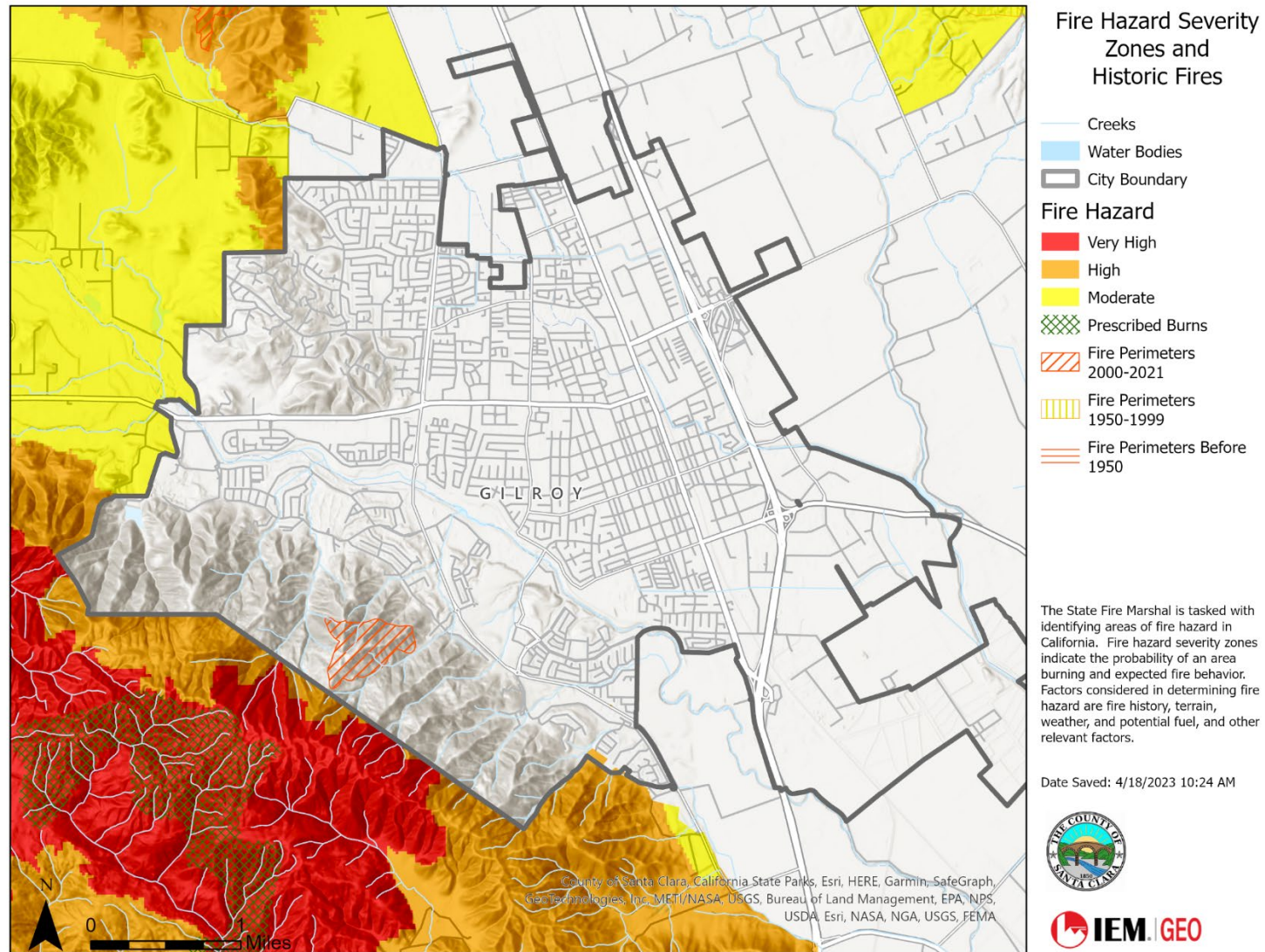
Figure 35: City of Gilroy Fire Hazard Severity Zones and Historic Fires
