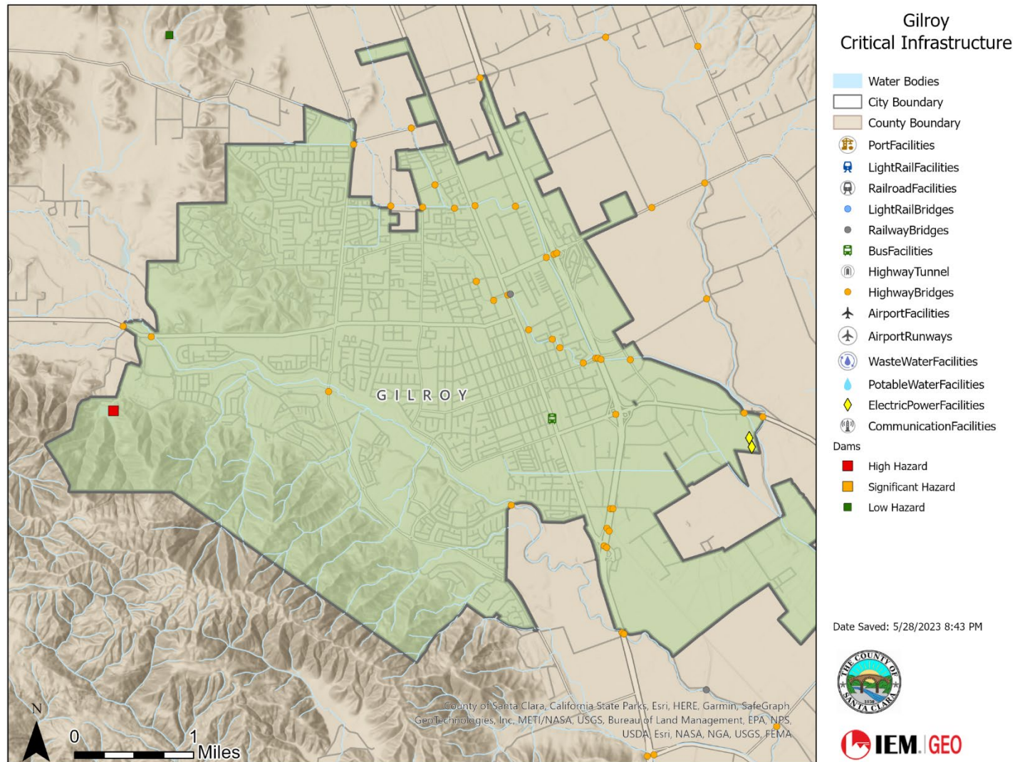
Figure 31: City of Gilroy Critical Infrastructure
