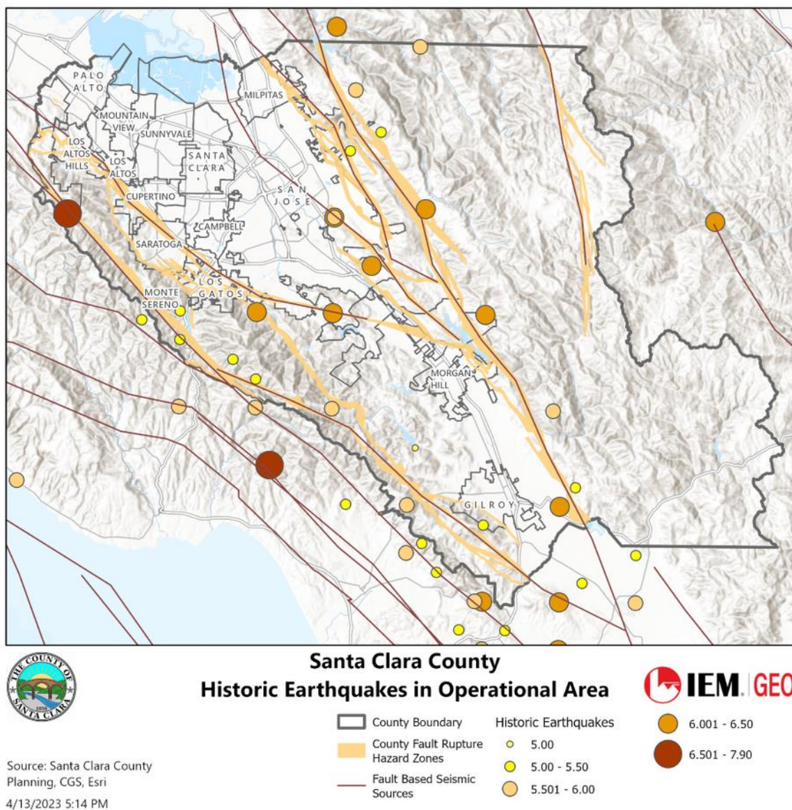
Figure 22: Historic Earthquakes in the Operational Area
