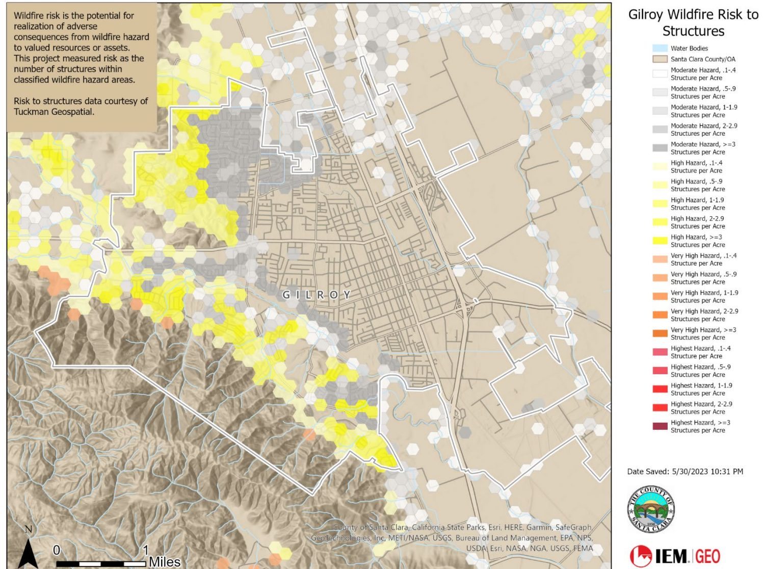
Figure 37: City of Gilroy Wildfire Risk to Structures Map
