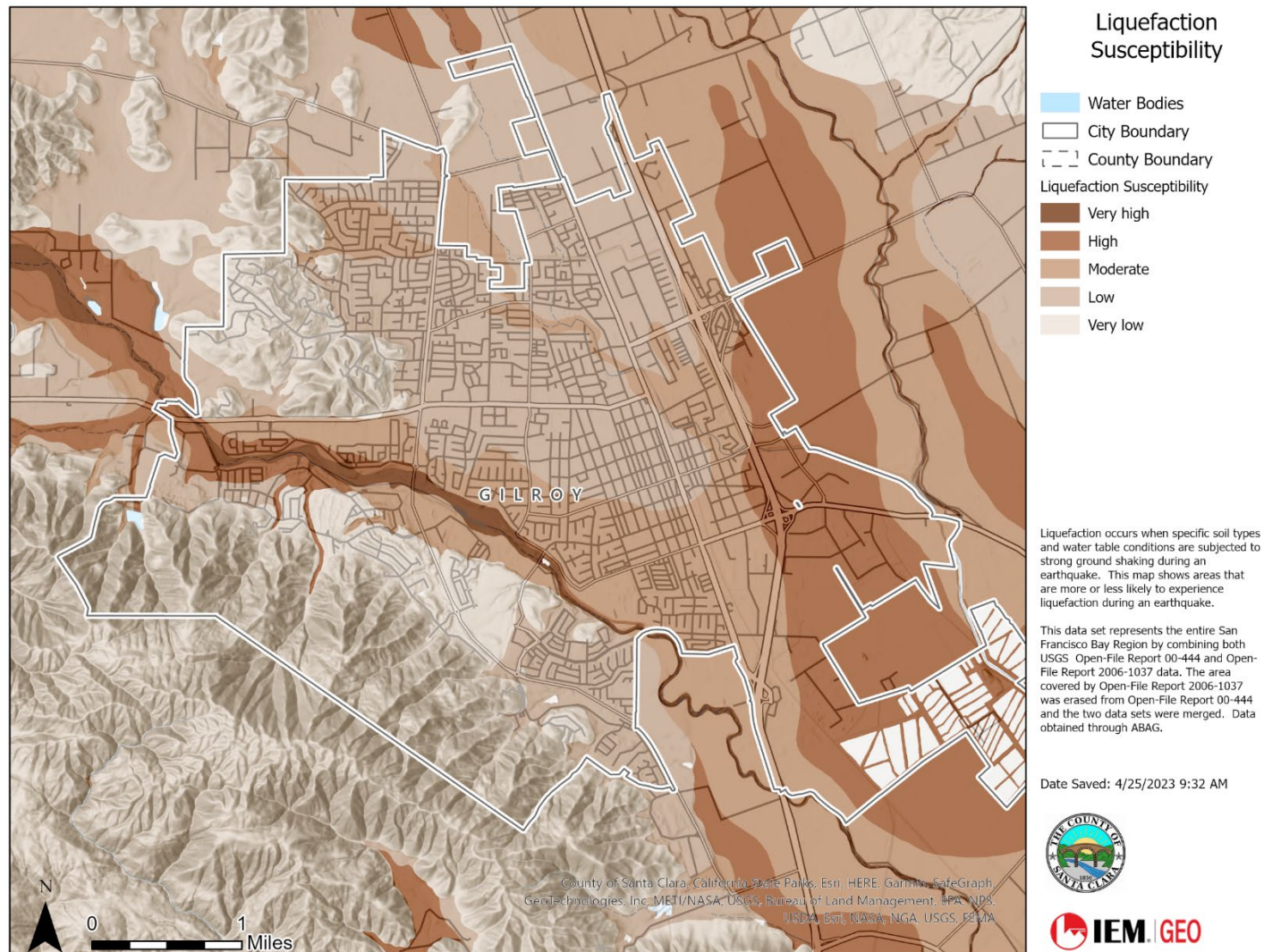
Figure 34: City of Gilroy Liquefaction Susceptibility Map
