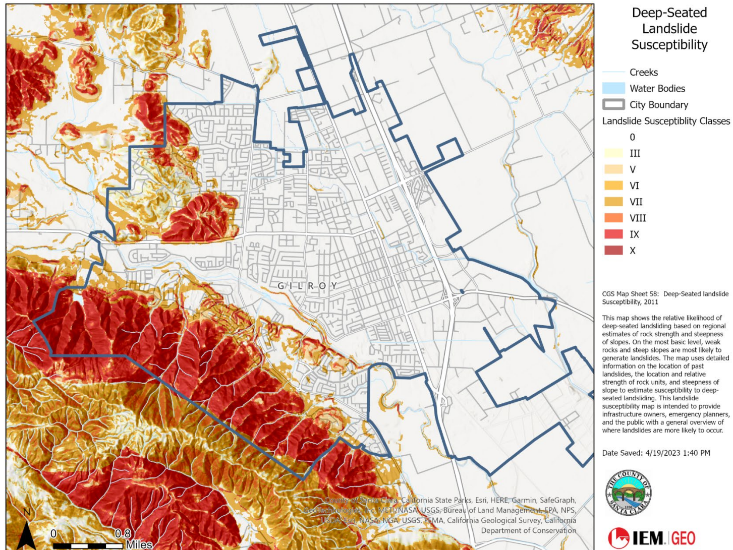
Figure 33: City of Gilroy Deep-Seated Landslide Susceptibility
