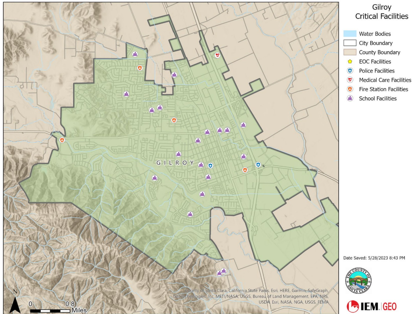
Figure 30: City of Gilroy Critical Facilities
